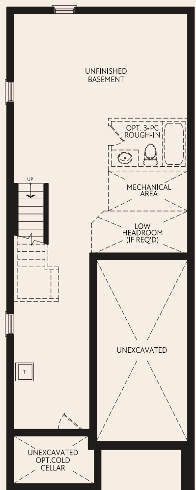
BASEMENT PLAN HERITAGE (C)
