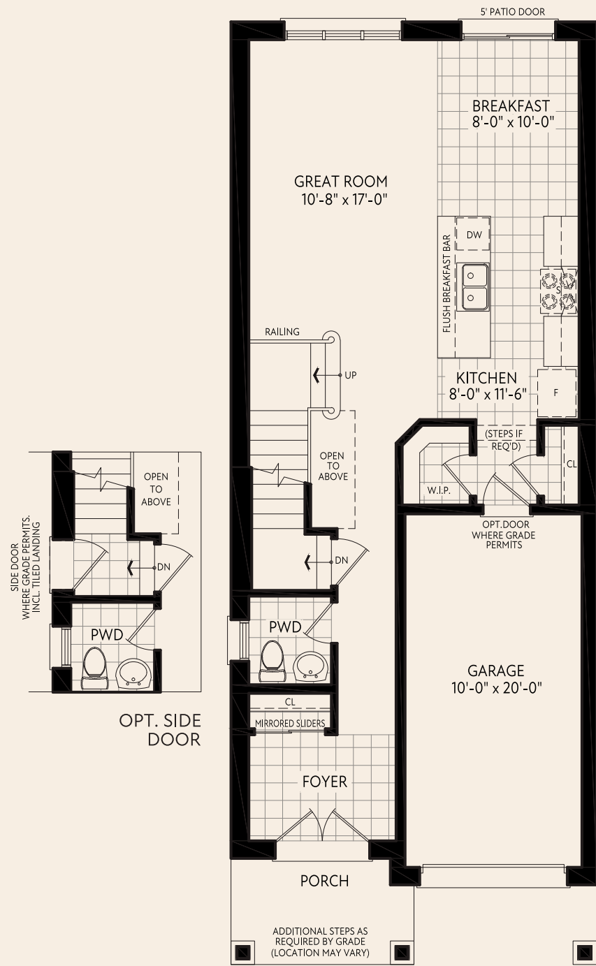
GROUND FLOOR PLAN HERITAGE (C)
