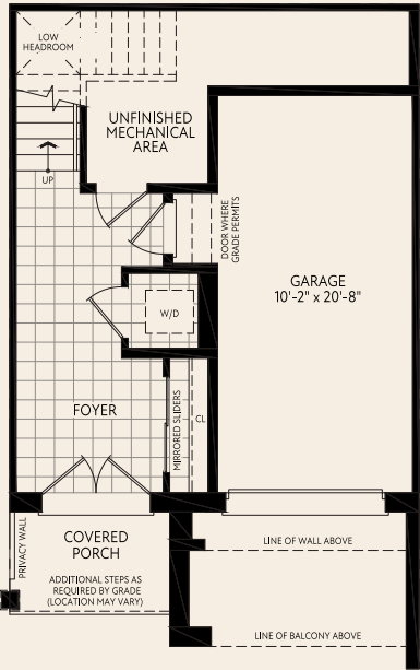
GROUND FLOOR PLAN MODERN (B)
