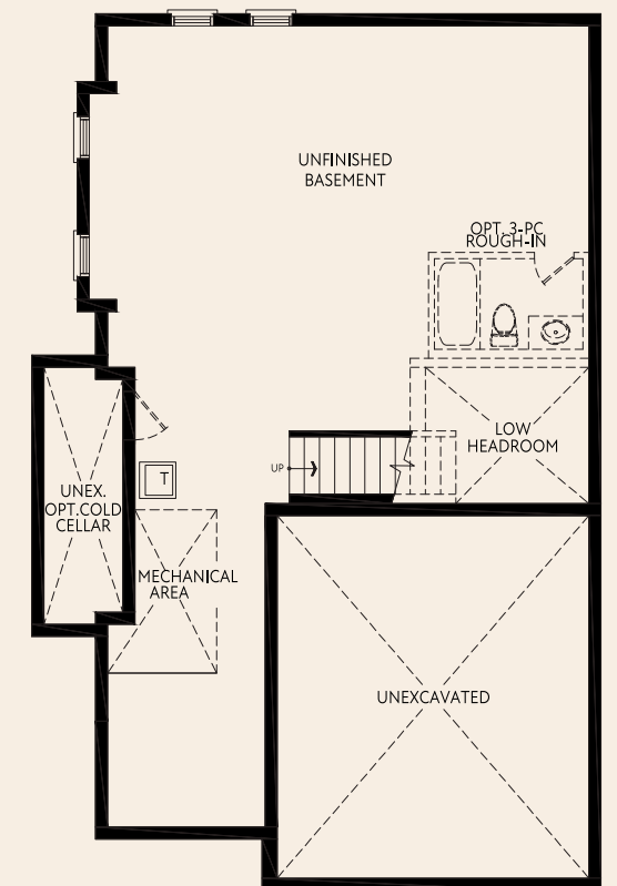
BASEMENT PLAN HERITAGE (C)
