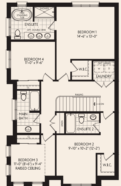
OPT. SECOND FLOOR PLAN HERITAGE (C)
