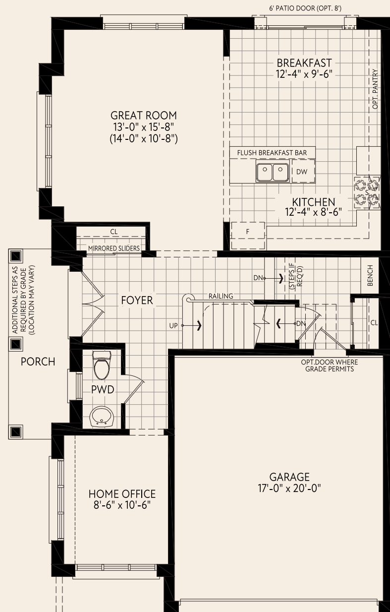
GROUND FLOOR PLAN HERITAGE (C)
