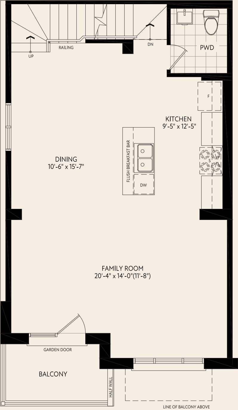
SECOND FLOOR PLAN MODERN (B)
