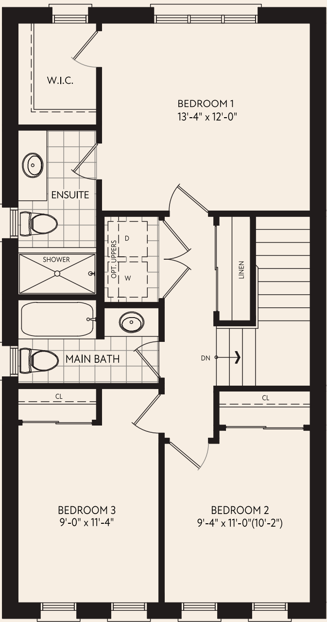
SECOND FLOOR PLAN HERITAGE (C)
