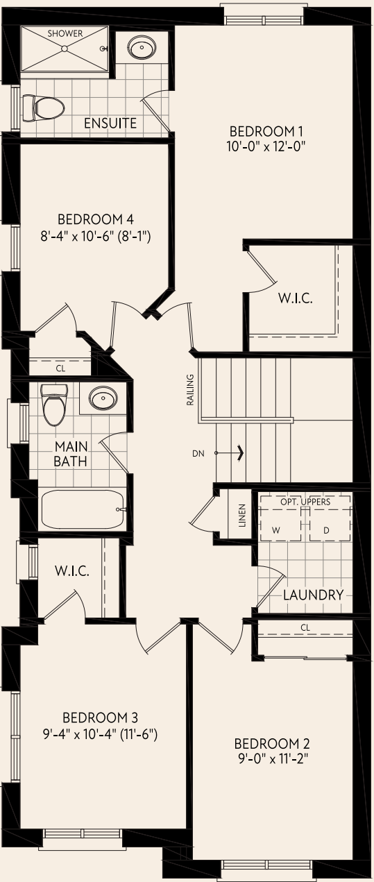
SECOND FLOOR PLAN OPT. 4 BEDROOM HERITAGE (C)
