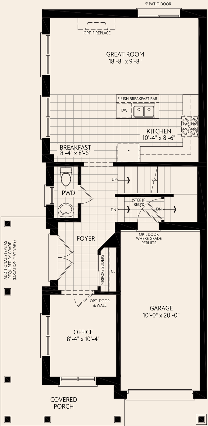
GROUND FLOOR PLAN HERITAGE (C)
