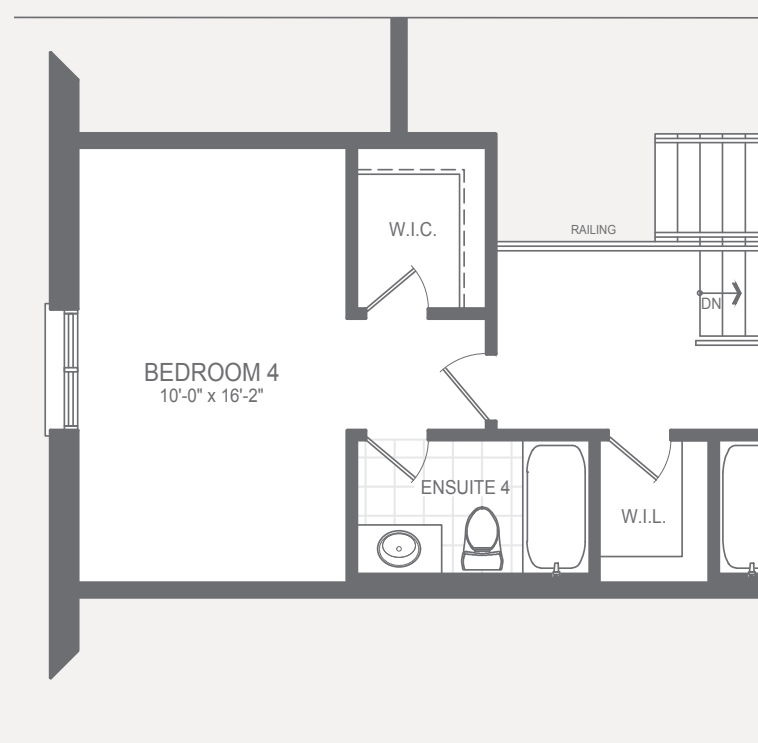
OPT. 4-BEDROOM LOFT FLOOR PLAN CLASSIC (A)
