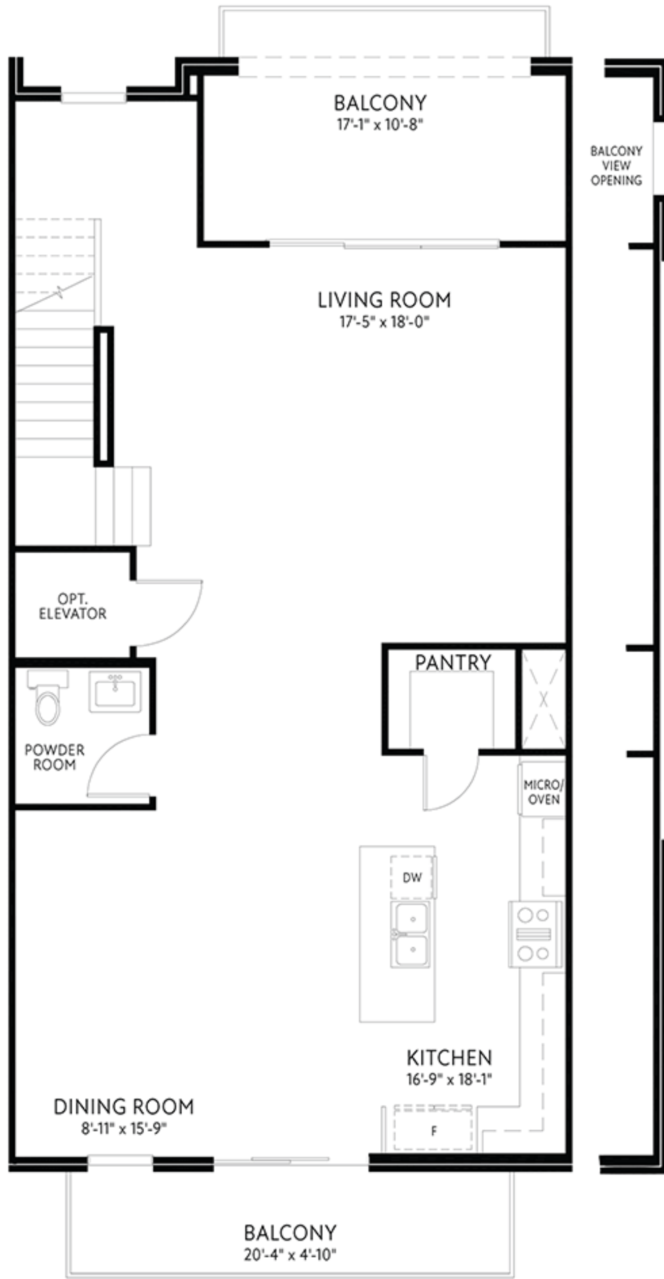
FLOOR 2
